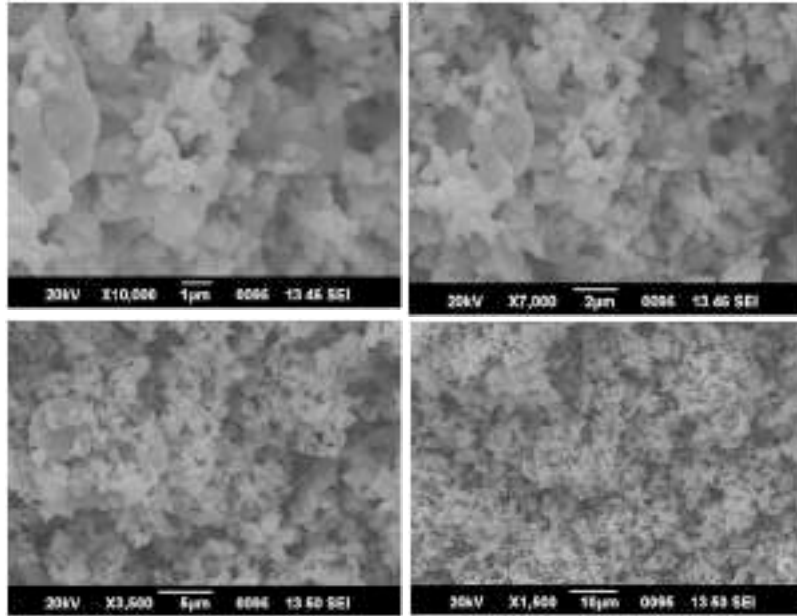
Fig.2. SEM images of sample \text{Sr}_{0.8}\text{Ba}_{0.2}\text{Fe}_{11.7}\text{La}_{0.2}\text{O}_{19}
